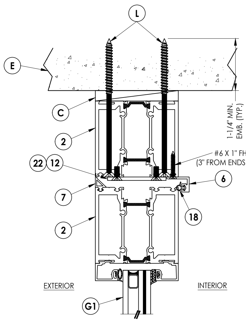
1 VERTICAL CROSS SECTION 6 Shown Direct to Masonry
