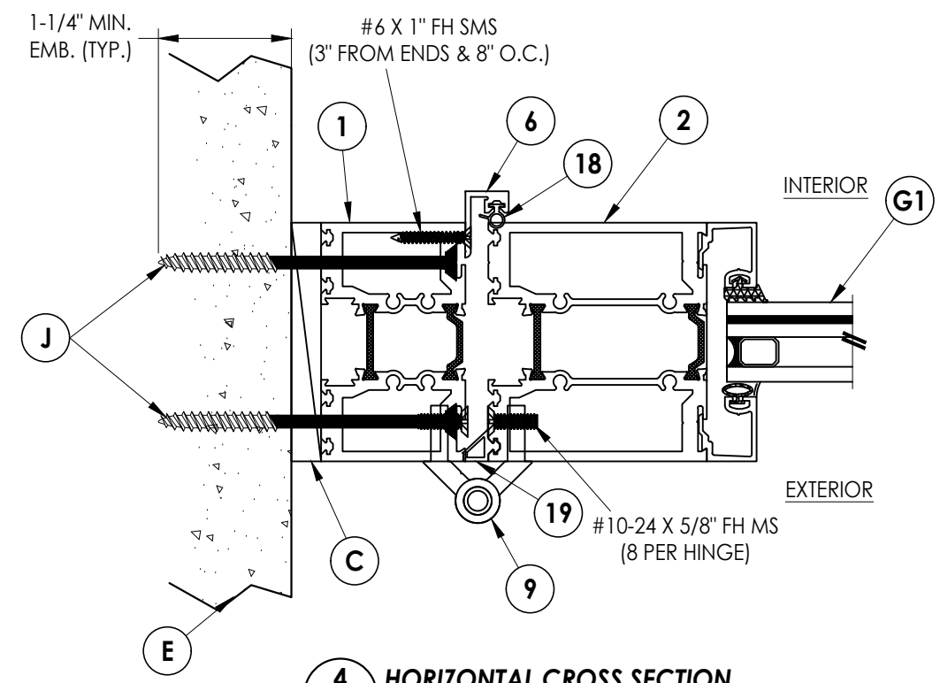
4 HORIZONTAL CROSS SECTION 6 Shown Direct to Masonry
