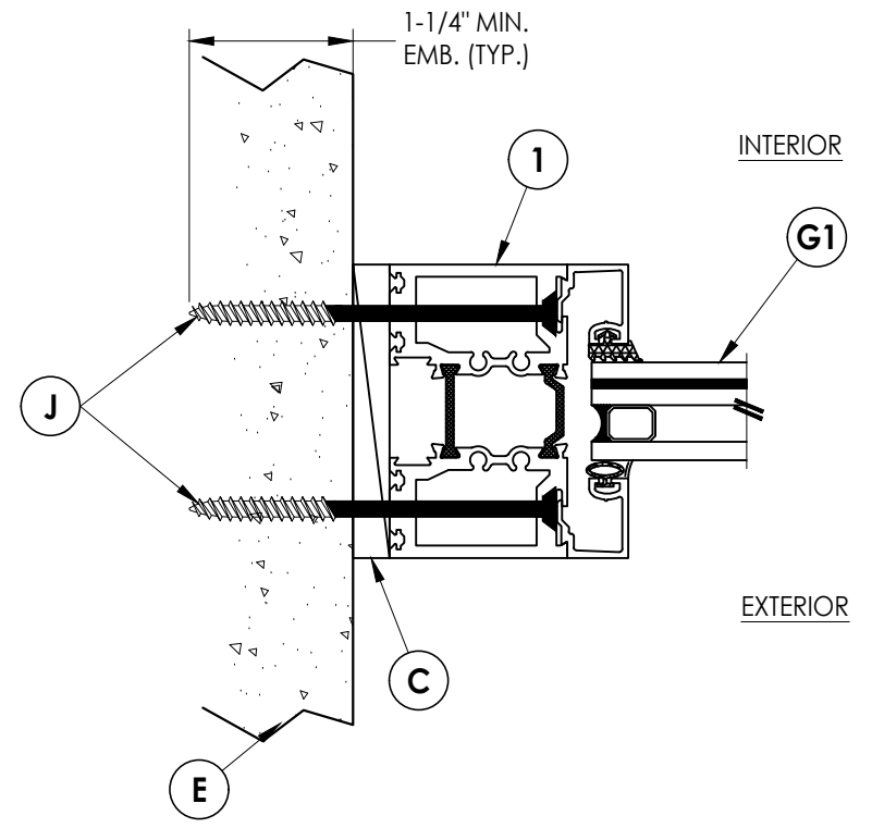
3 HORIZONTAL CROSS SECTION 6 Shown Direct to Masonry
