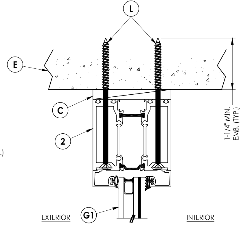
2 VERTICAL CROSS SECTION 6 Shown Direct to Masonry
